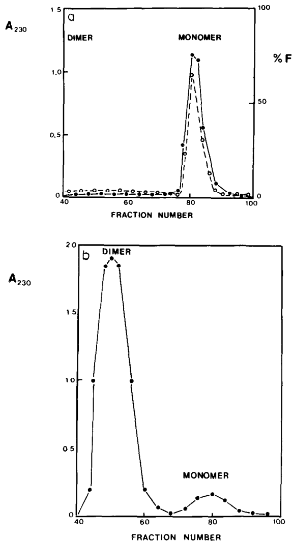
Fig.1.(a) Sephadex G-100 chromatography of iodozobenzoate-treated IAEDANS-labelled histone H3, (H3-(Cys-IAEDANS)). Eluant: 50 mM NaCl, 50 mM acetate (pH 5.1). (●—●), A_{230} (○—○) fluorescence. (b) Sephadex G-100 chromatography of unlabelled histone H3 after treatment with iodozobenzoate. Conditions as for a.
