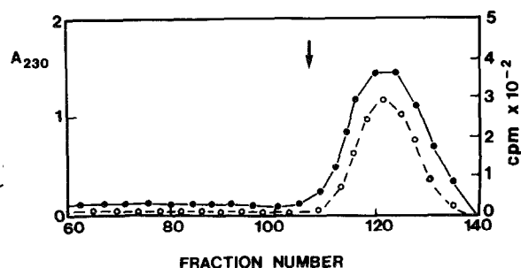
Fig.3. Attempted reconstitution of histone octamers from H3 labelled with iodo[ ^{14}\text{C} ]acetamide and subsequently treated with iodosobenzoate and chromatographed on a Sephadex G-100 column to remove dimerised unsubstituted material. The absence of an aggregate peak is explained by the precipitation of 35% of the radioactivity during octamer reconstitution. Conditions as for fig.2. ( \bullet — \bullet ) A_{230} , ( \circ — \circ ) cpm.
